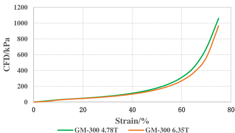
GM-300 Compression force deflection curve
